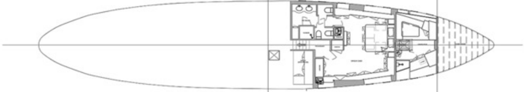
LOWER DECKS
