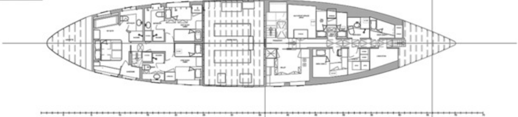
LOWER DECKS
